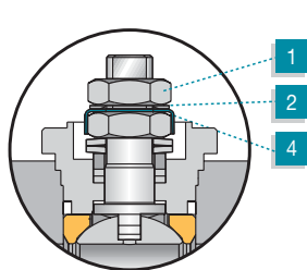
Actuated Valve stem assembly
