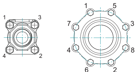
FIGURE 6 Body Bolt Tightening Pattern
